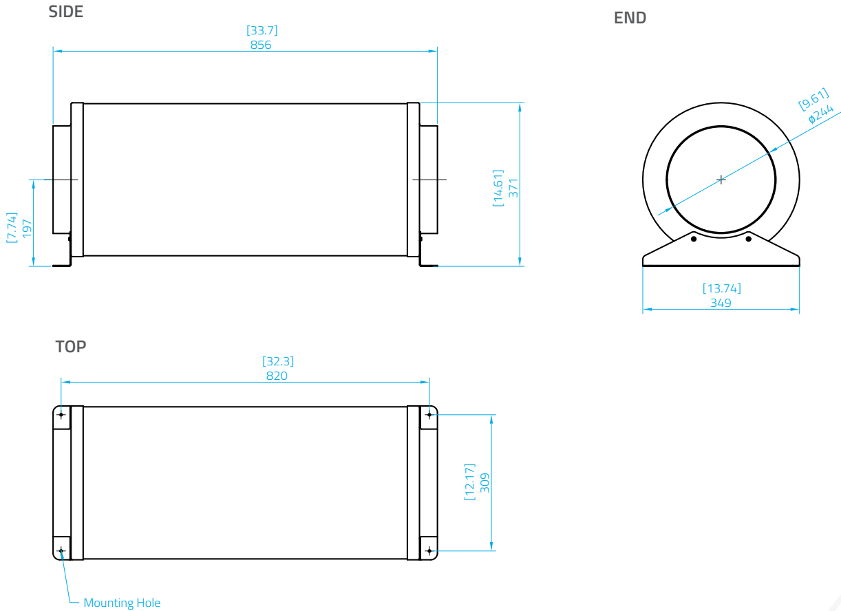
Mistral 250 - technical drawing
