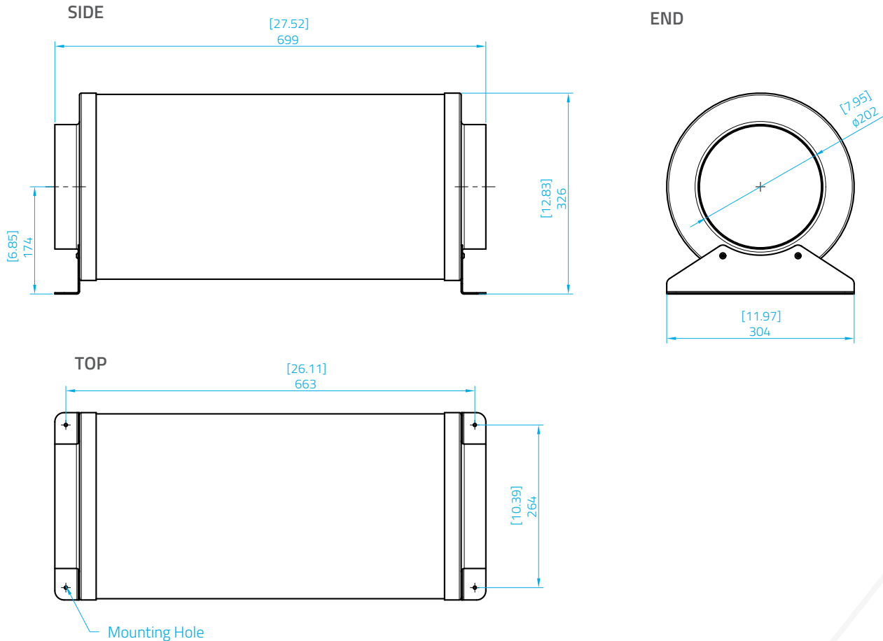
Mistral 200 - technical drawing
