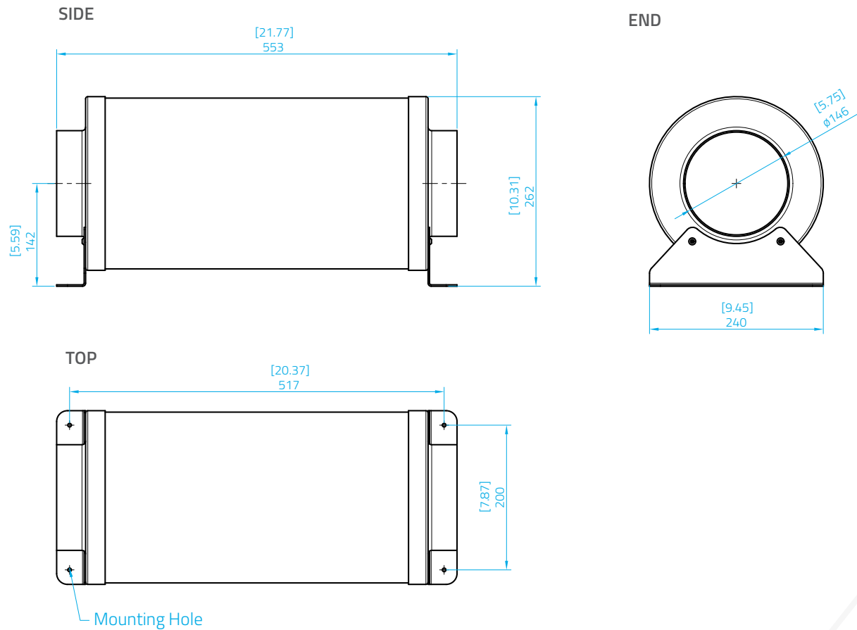
Mistral 150 - technical drawing
