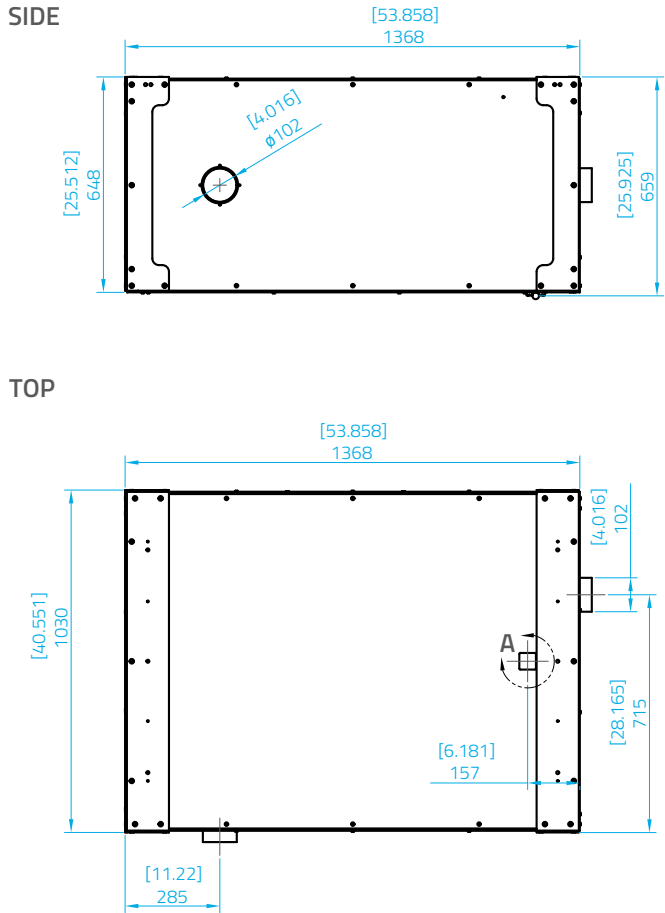
Hush Box Large with Side Ports for Athena projector model - technical drawing
